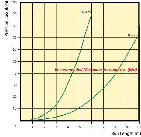
Drip Eze™ 2.0L/h Pressure Loss Chart
