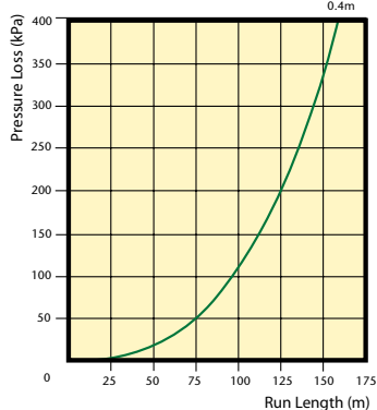
Drip Eze™ 1.6L/h Pressure Loss Chart
