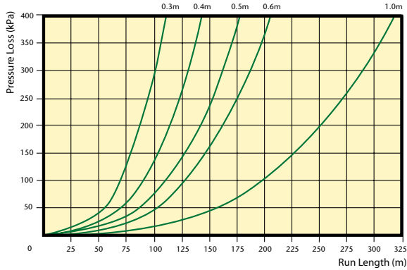
Drip Eze™ 1.6L/h Pressure Loss Chart
