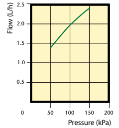
Flow v Pressure Chart
