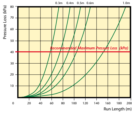
Drip Eze™ 2.0L/h Pressure Loss Chart
